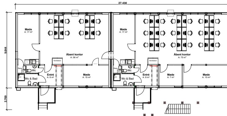
Plan 1 1:200
