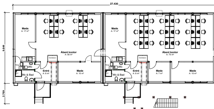
Plan 1 1:200
