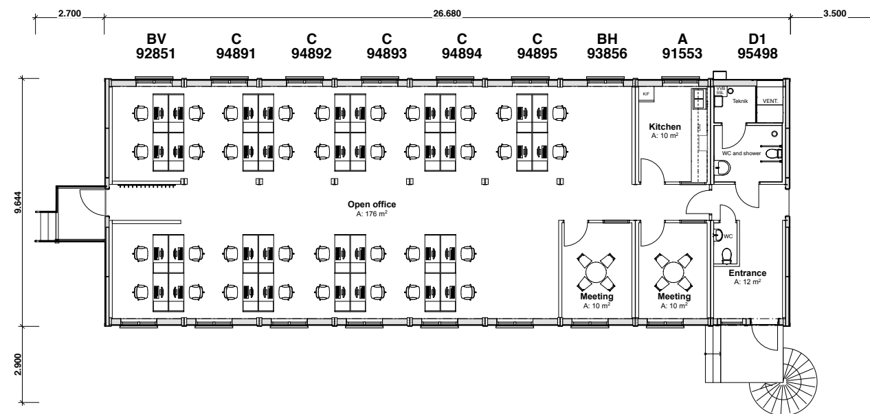
Plan 2 1:200
